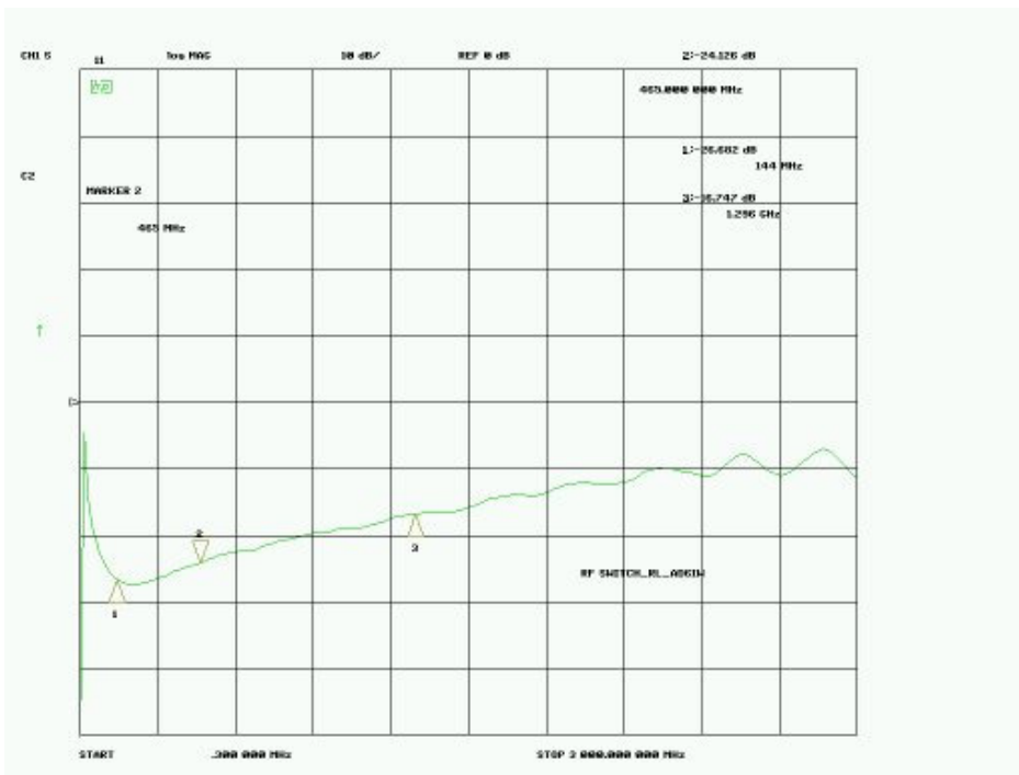
Figure 6 Return loss
