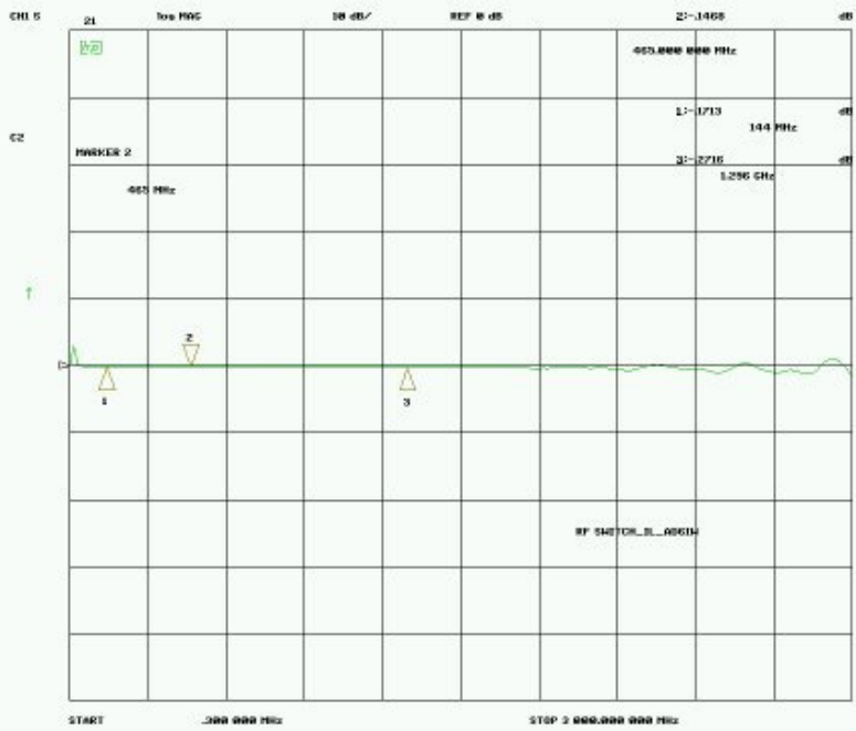
Figure 4 Insertion loss
