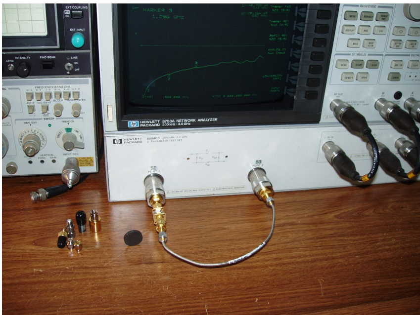
Figure 3 Switch testing
