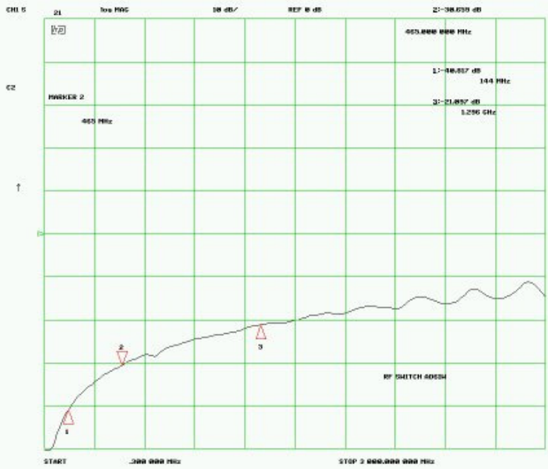
Figure 5 Isolation
