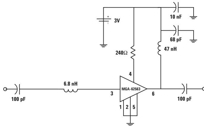
Figure 1a. Test circuit of the 0.5 GHz production test board used for NF, Gain and OIP3 measurements. This circuit achieves a trade-off between optimal NF, Gain, OIP3 and input return loss. Circuit losses have been de-embedded from actual measurements.
