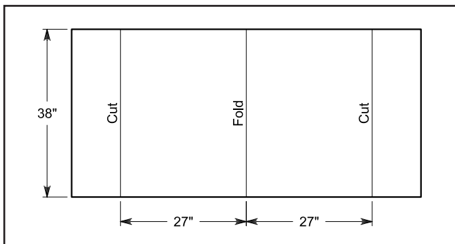
Figure 10—Cutting instructions for the high-performance corner reflector surfaces.
