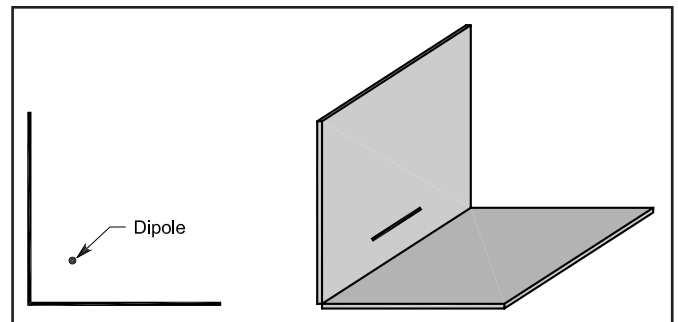
Figure 6—The basic corner reflector used for the uplink antenna. Note the dipole feed.
