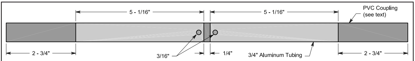
Figure 7—Dimensions for the corner reflector dipole feed.
