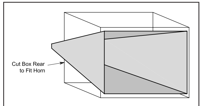
Figure 3—The final downlink antenna assembly showing how the horn fits into the supporting carton.
